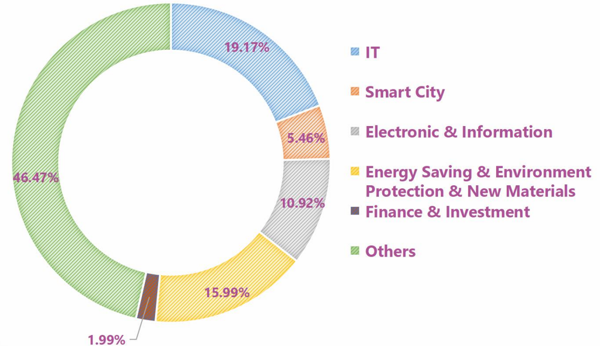
Specialty Breakdown
