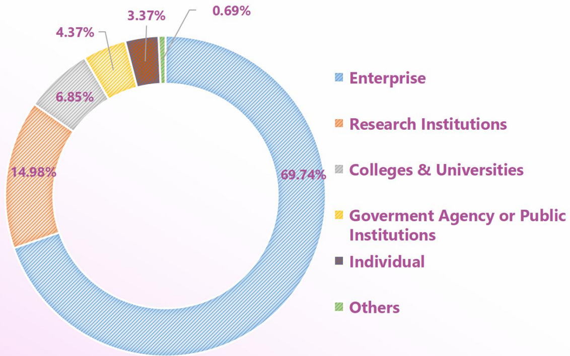
Exhibitor Breakdown
